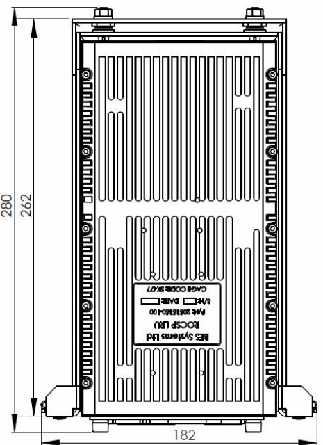
FDR-1000 with a tray, dimensions
